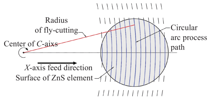
(b) ZnS 晶体表面圆弧形加工轨迹 (b) Circular arc process path on ZnS element
