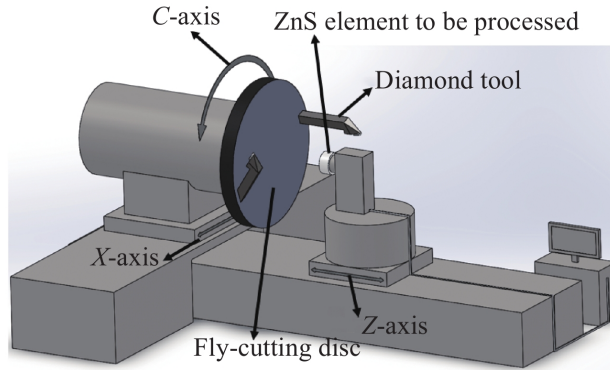
(a) 飞刀加工模型 (a) Model of fly-cutting
